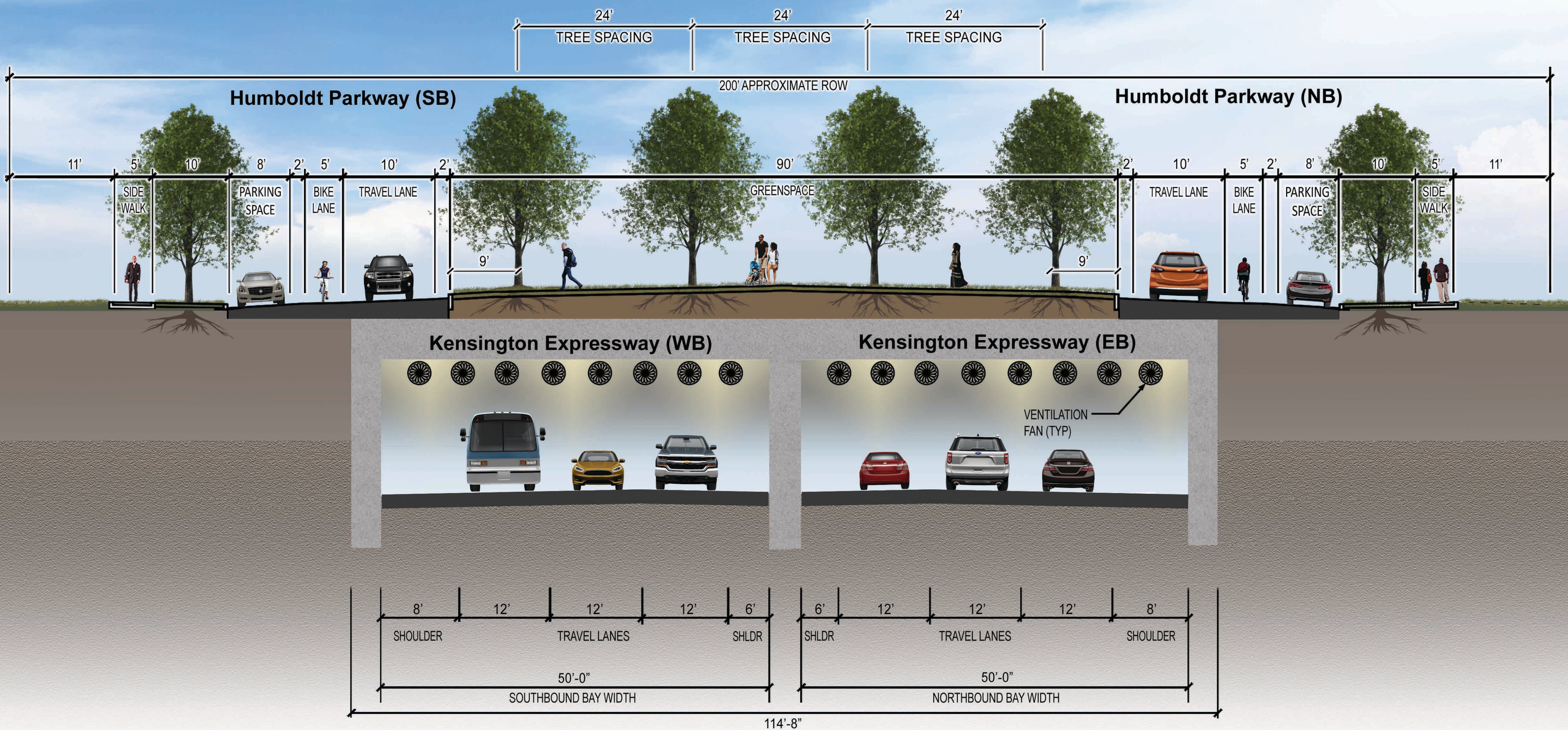
SECTION H-H PROPOSED CORRIDOR UNDER BUILD ALTERNATIVE
